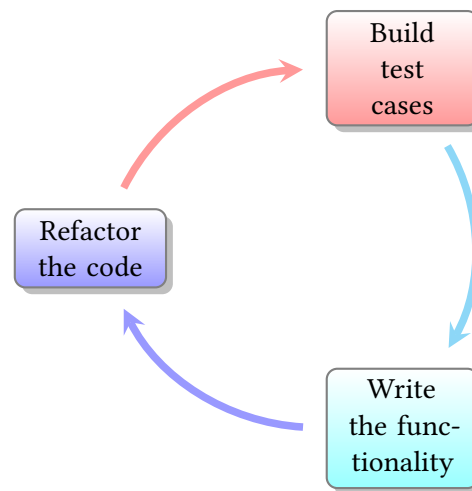
Figure 2.3: TDD cycle
